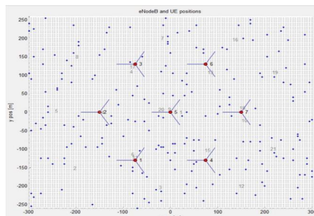
Figure.9 5G nodes & UE map with 150m inter-node-distance, and 210 UEs (dark dots) with 10 UEs per cell
