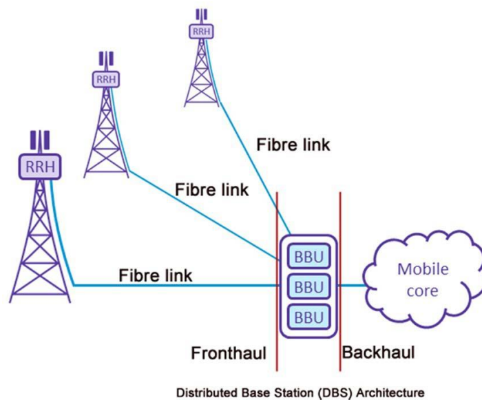
Figure.1 Distributed Base Station Architecture.
