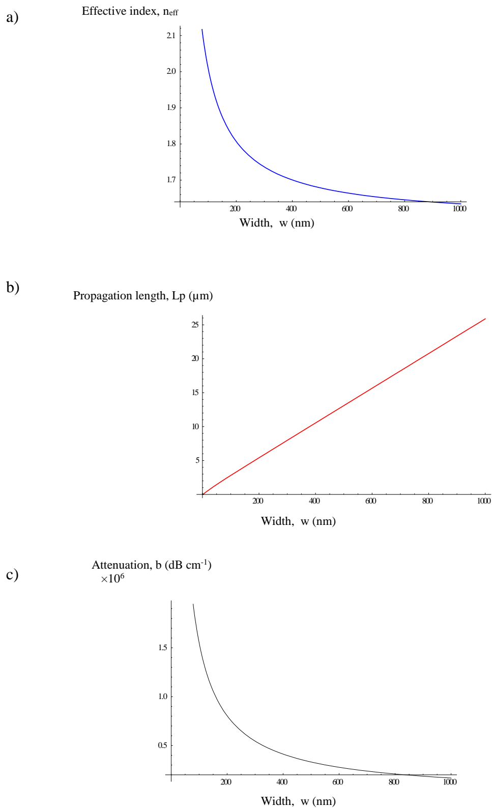
Figure.4: The effective index n_{\text{eff}} , propagation length L_p , and the attenuation b , as functions of width of the gap of the E7 w for \lambda=633 nm (MIM plasmonic waveguides Ag/E7/Ag, \epsilon_d = 2.5363 and silver metal \epsilon_{\text{Ag}} = -14.4688 - i 1.09378 .)
