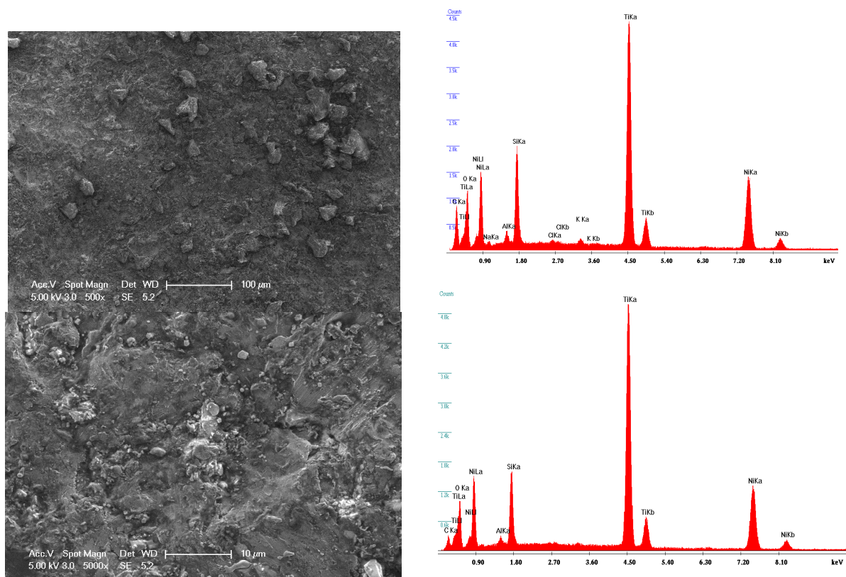
Figure. 6. Micrographs from the worn surfaces of unreinforced TiNi produced at T=1200^{\circ}\text{C}
