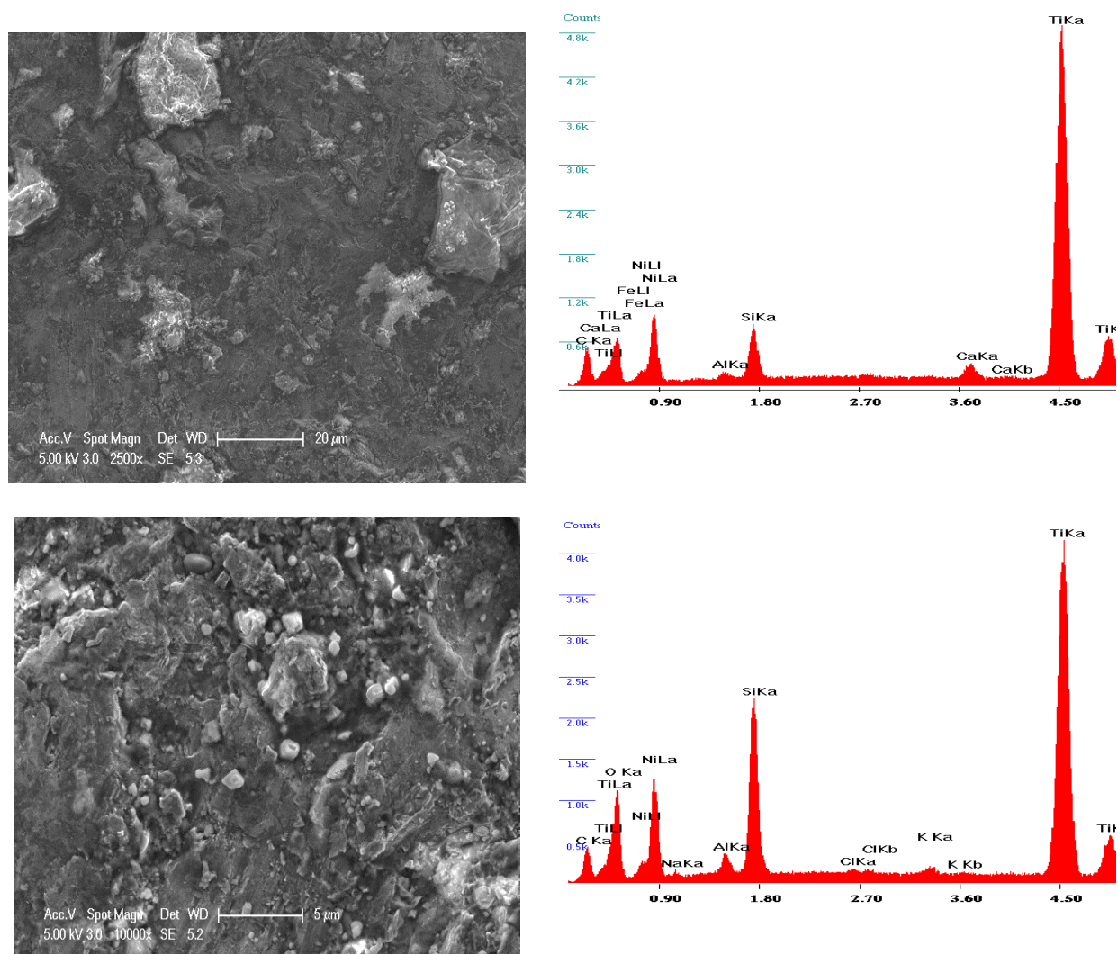
Figure. 7. FESEM micrographs from the worn surfaces of TiNi-CNTs nanocomposites produced at T=1200^{\circ}\text{C} reinforced with 0.8 wt% SWCNTs
