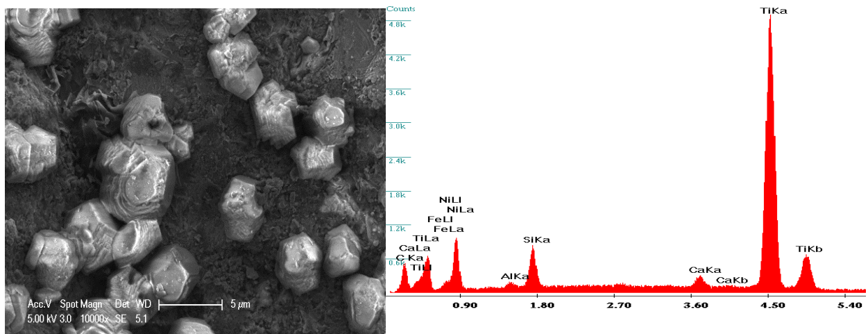
Figure. 6. Micrographs from the worn surfaces of unreinforced TiNi produced at T=1200^{\circ}\text{C}
