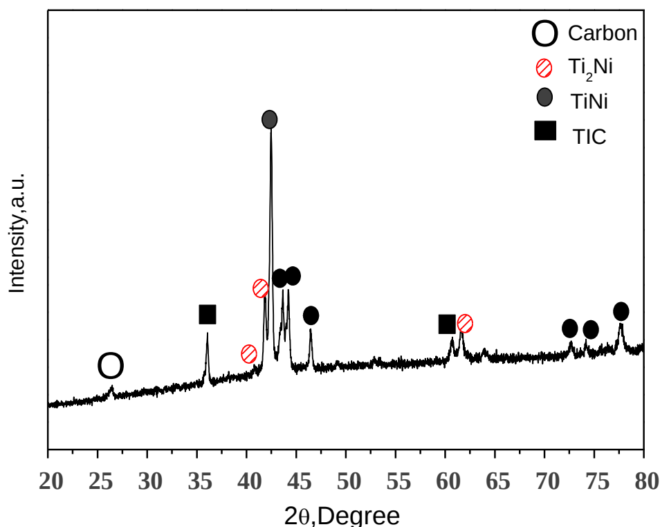
Figure. 4. XRD spectra of reinforced TiNi-CNTs nanocomposites produced at T=1200^{\circ}\text{C} reinforced with 0.8 wt% SWCNTs (SPS 2 )
