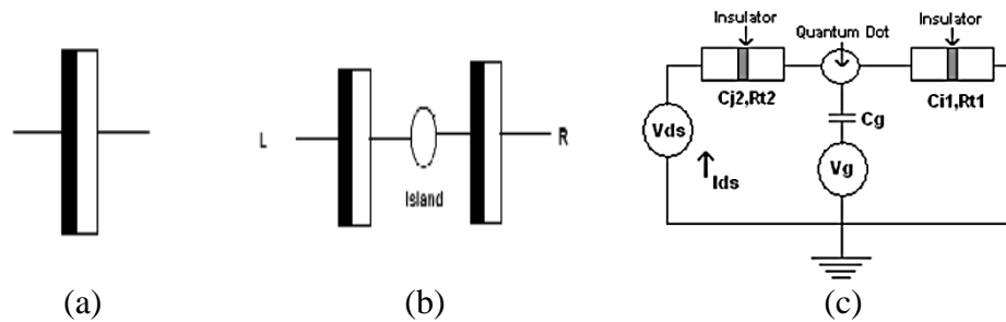
Figure. 1: (a) Schematic diagram for a tunnel junction, (b) Quantum dot island with two tunnel junctions, (c) Circuit diagram of the Single Electron Transistor.
